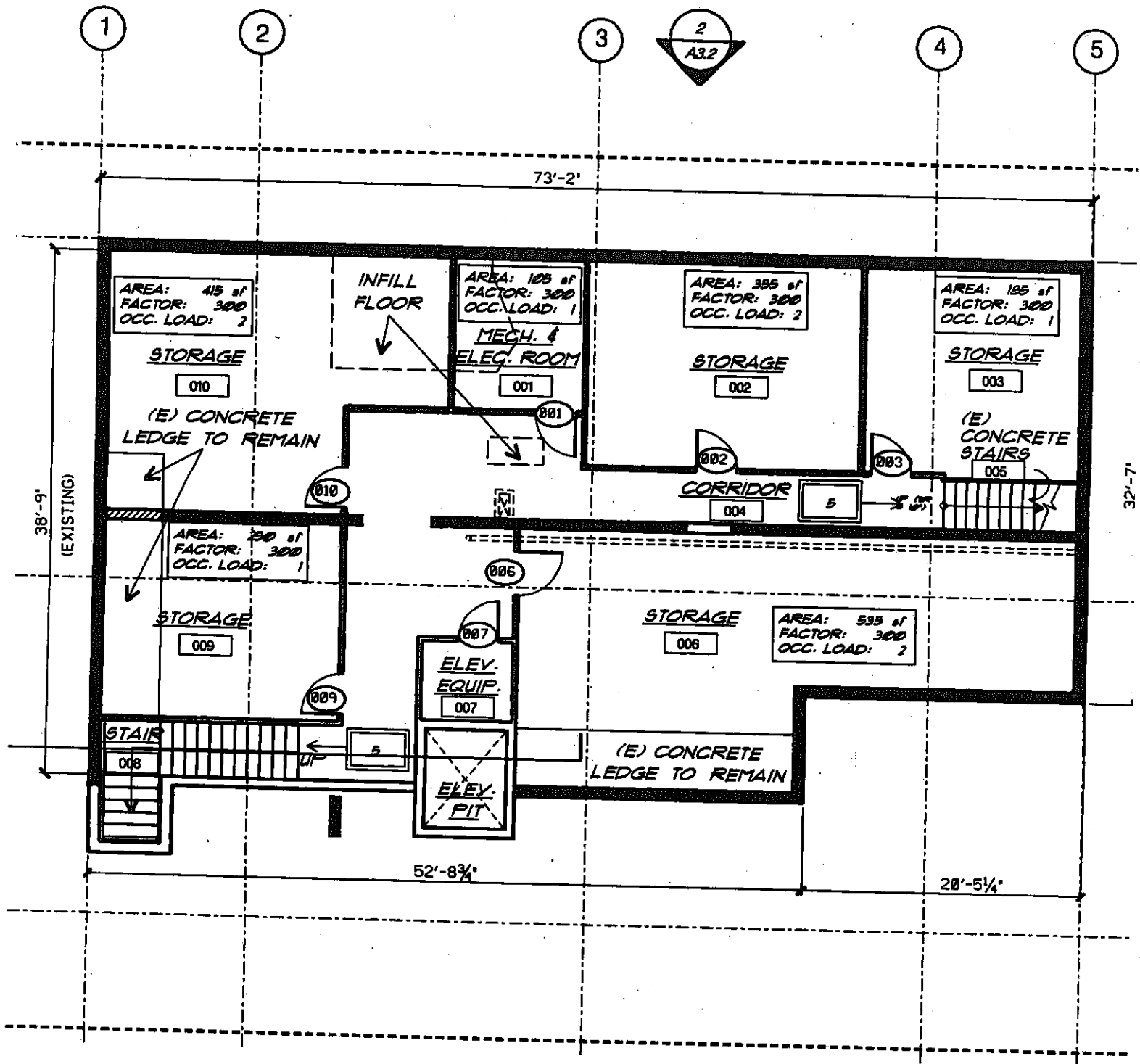
1 BASEMENT FLOOR PLAN 1/8" = 1'-0" 2300 SF (NET)
